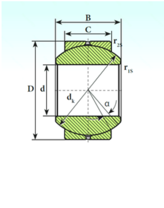
GE 10 SB Bearing 2D drawings and 3D CAD models
